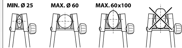
ART. 319C - 319CP CHIUSURA CON POMELLO CLOSE-UP WITH KNOB
